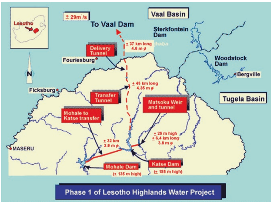
Fig. 1 Phase 1 of Lesotho Highlands Water Project. (Source: Letsebe 2012)
