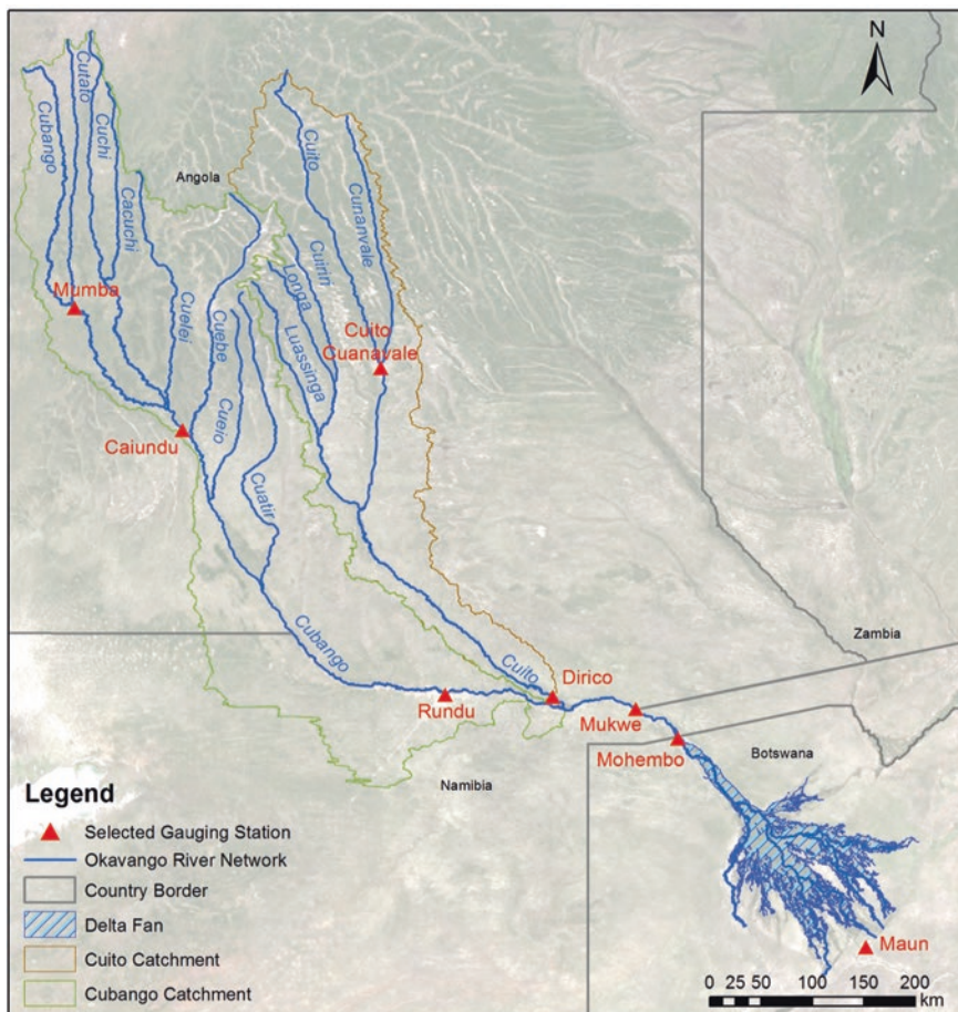
Fig. 1 Okavango River Basin including the main tributaries, flow gauging stations and the Okavango Delta with its entrance at Moheumbo gauging station and outlet at Maun (Data source: NIWR, ORI; background, MODIS 16-day BRDF-adjusted NBAR data (MCD43A4) courtesy of EOSDIS-NASA) in Steudel et al. 2013
